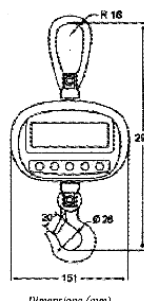
Dimensions (mm)
